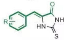
19a-19c (thiohydatoin)
